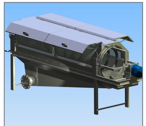
Rotating drum view
